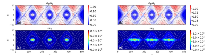
Fig. 8. The energy distribution of particles in squashed magnetic islands at t = 560 \Omega_{ci}^{-1} . The initial electric field comes from Eq.(8). The other physical parameters are identical to the simulation in Fig.6.
