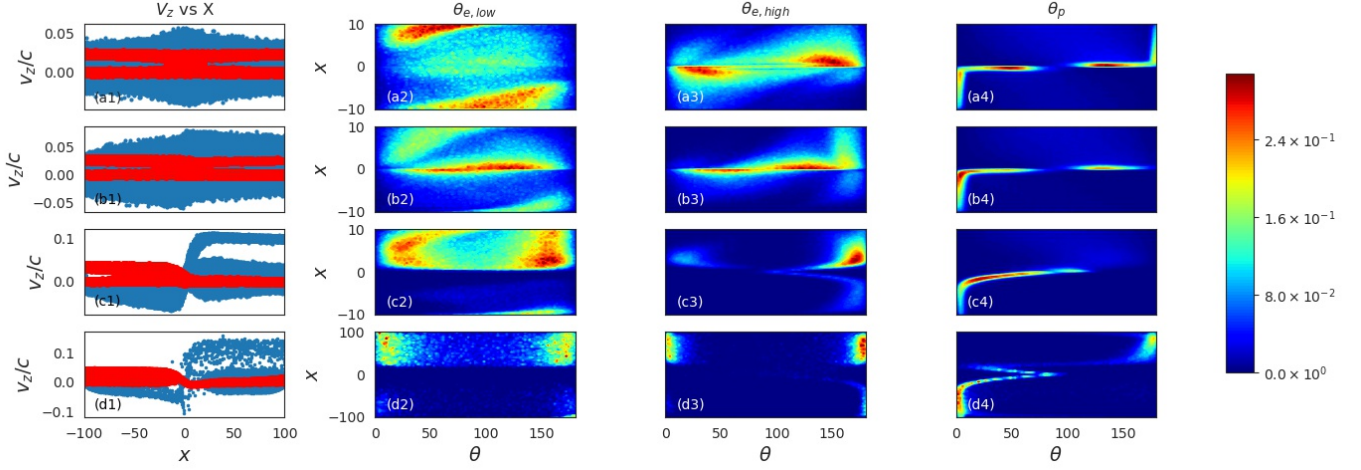
Fig. 4. The V_z vs x distributions in phase space and the pitch-angle distributions for B_y/B_0 = 0 (a-first row), 0.1(b-second row), 1.0(c-third row), and 1.0 with d = 10 (d-fourth row): In each row, V_z vs x of electrons (blue dots) and protons (red dots) (first column), the pitch-angle distribution of low-energy electrons (second column), the pitch-angle distribution of high-energy electrons (third column), and the pitch-angle distribution of protons (fourth column) are presented from left to right for each individual B_y/B_0 ratio. The current sheet parameters are B_0 = 10^{-3} T , E_0 = 250 V/m , and d = 1 for (a-c). The magnetic field topology in the reconnection plane is similar to Fig.1.
