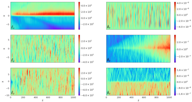
Fig. 2. The changes of electric and magnetic fields in the simulation ( n_0 = 10^{10} m^{-3} ): the left column shows the x, y, z components of \vec{\mathbf{E}} (in the unit of V/m ), and the right column is for \vec{\mathbf{B}} (in T ) at t = 70\Omega_{ci}^{-1} .
