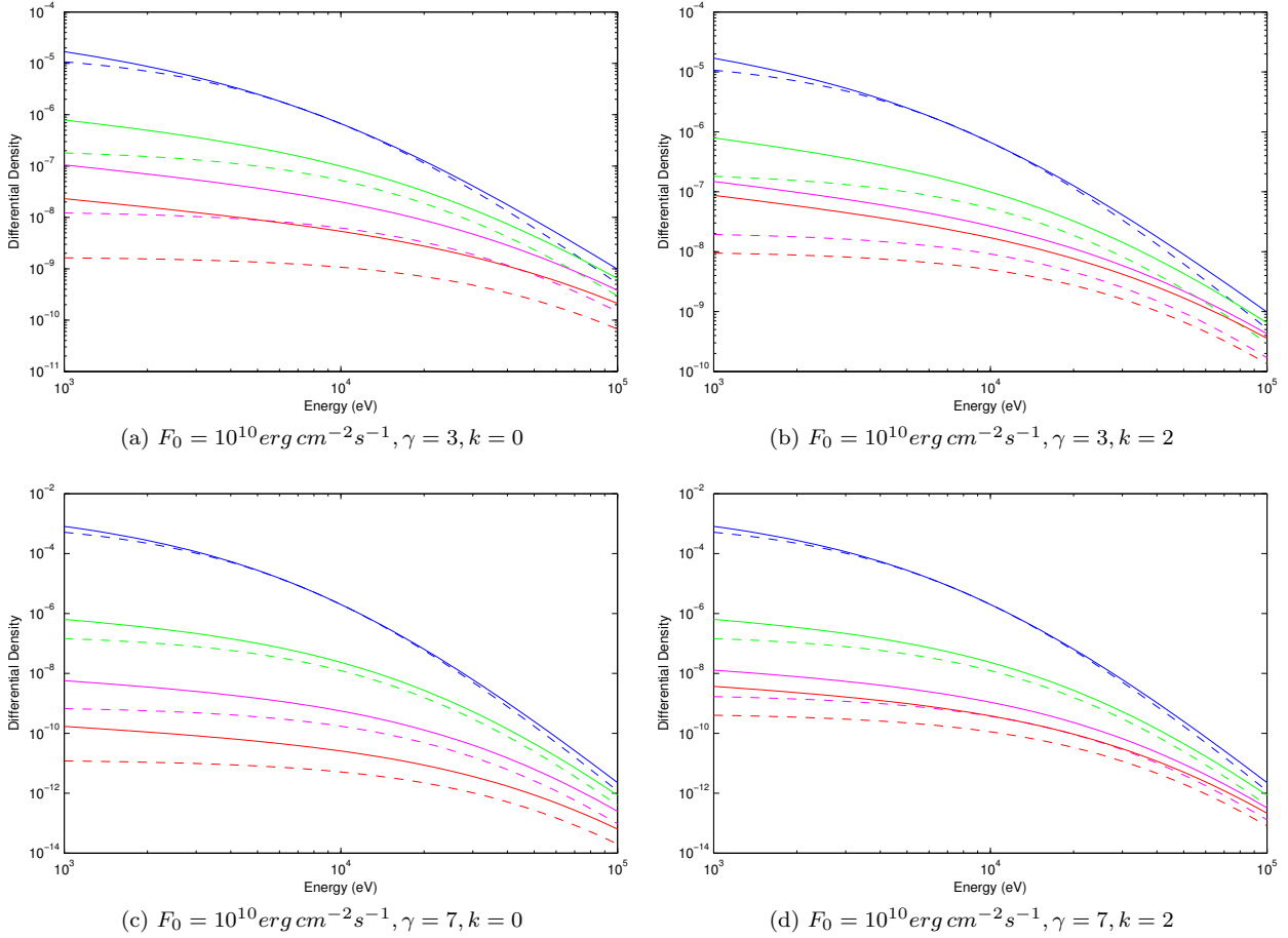
Figure 2. The variations of beam electron differential density vs. energy calculated, at the precipitation depths ( s ) of 1.6 \times 10^8 \text{ cm} (blue), 4.8 \times 10^8 \text{ cm} (green), 9.6 \times 10^8 \text{ cm} (magenta) and 16.0 \times 10^8 \text{ cm} (red). The solid lines represent the results of the updated CE (equation 40) and the dashed lines correspond to the original approach (equation 28) by Zharkova & Gordovskyy (2006).
