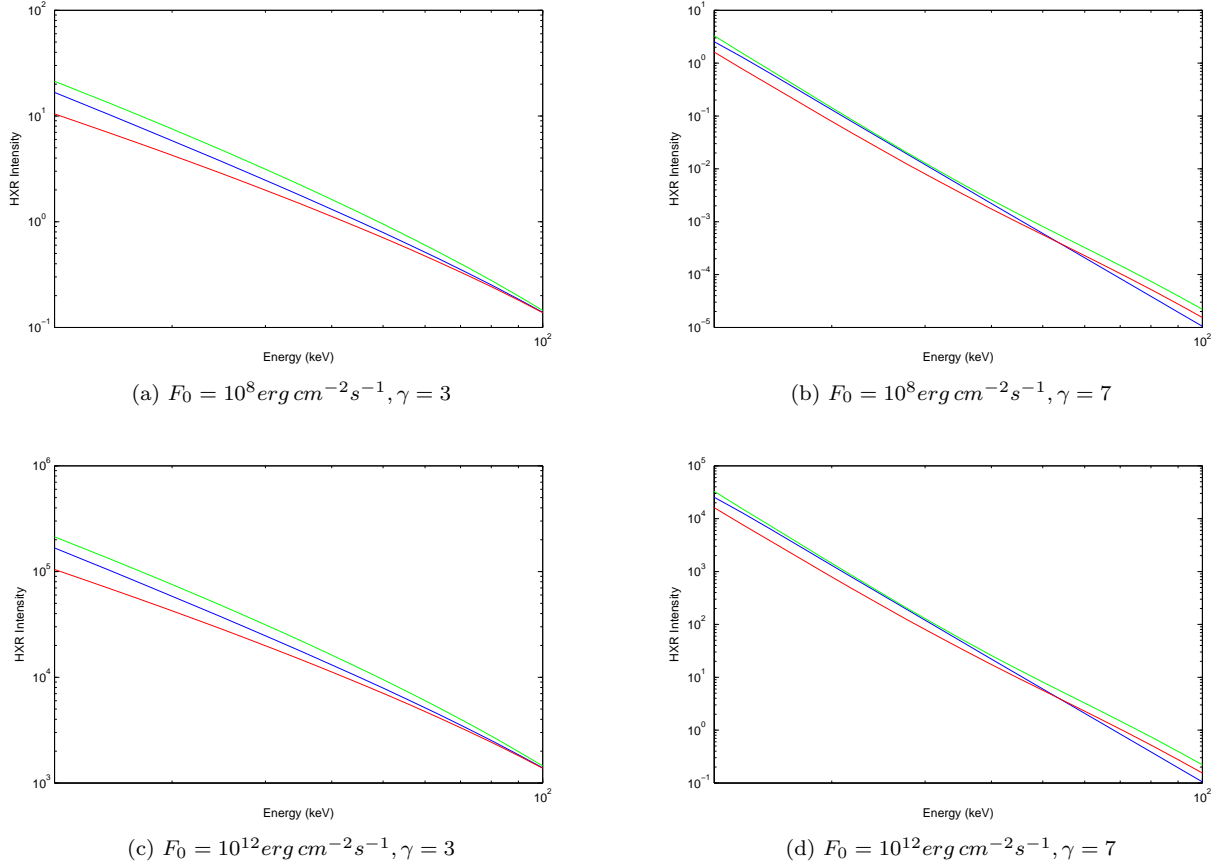
Figure 4. Hard X-ray intensity in relative units, obtained from the original CE (red lines), the updated CE (green lines) solution for purely Coulomb collisions and the numerical Fokker-Planck solution (blue lines).
