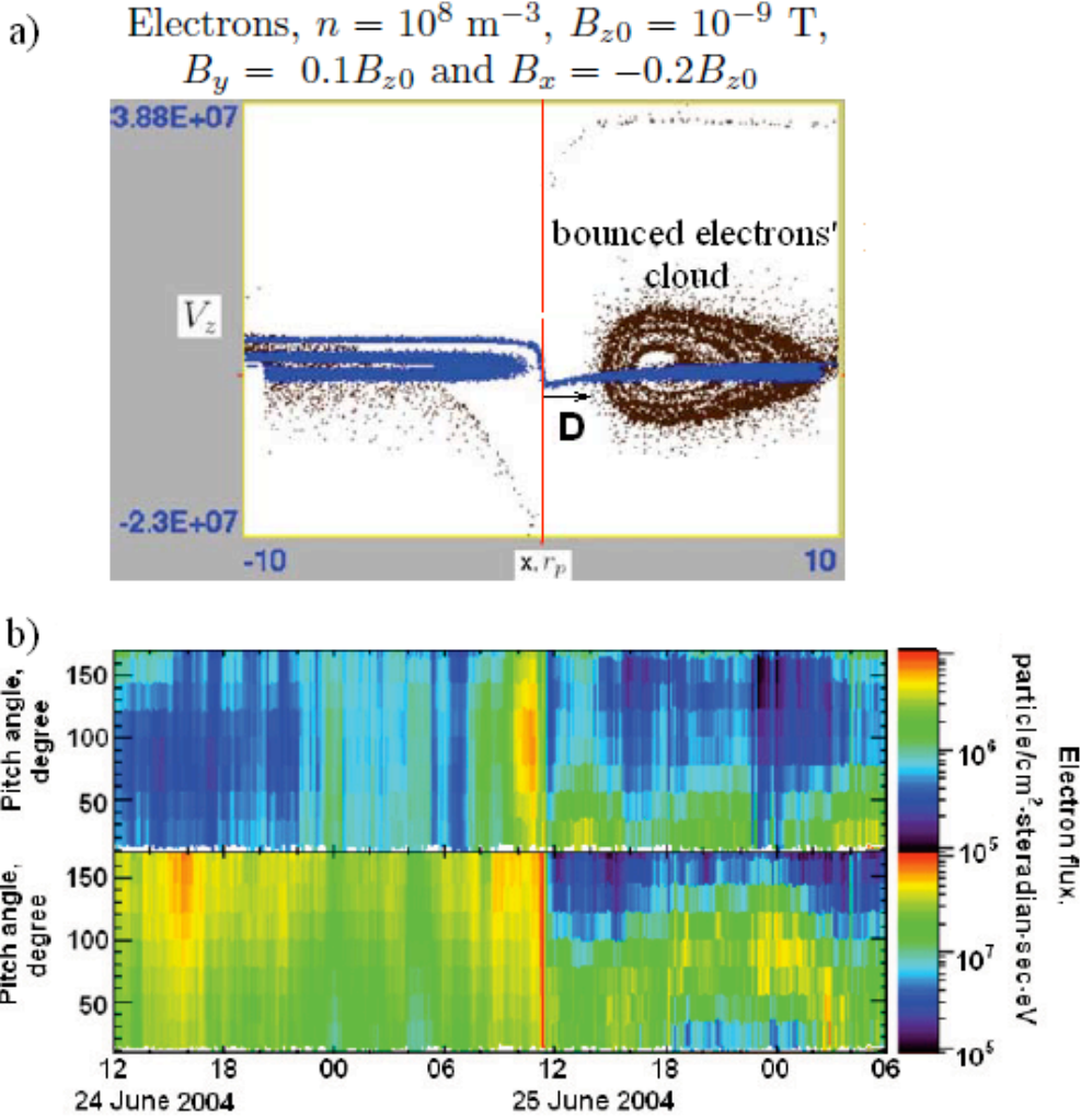
Figure 1. Comparison of a) accelerated electron (black dots) and proton (blue dots) distributions simulated for strong guiding field with PIC with respect to the current sheet midplane ( X=0 ) and b) observed energy and pitch angle distributions of electrons passed through the HCS. Note that simulated distributions of the bounced electrons (for X > 0 ) do not reach the midplane but turned back at some distance D from it. This causes the pitch angle distributions shown in b) with the variations of a pitch angle from 0 to 180^\circ similar to the simulated variation in a).
