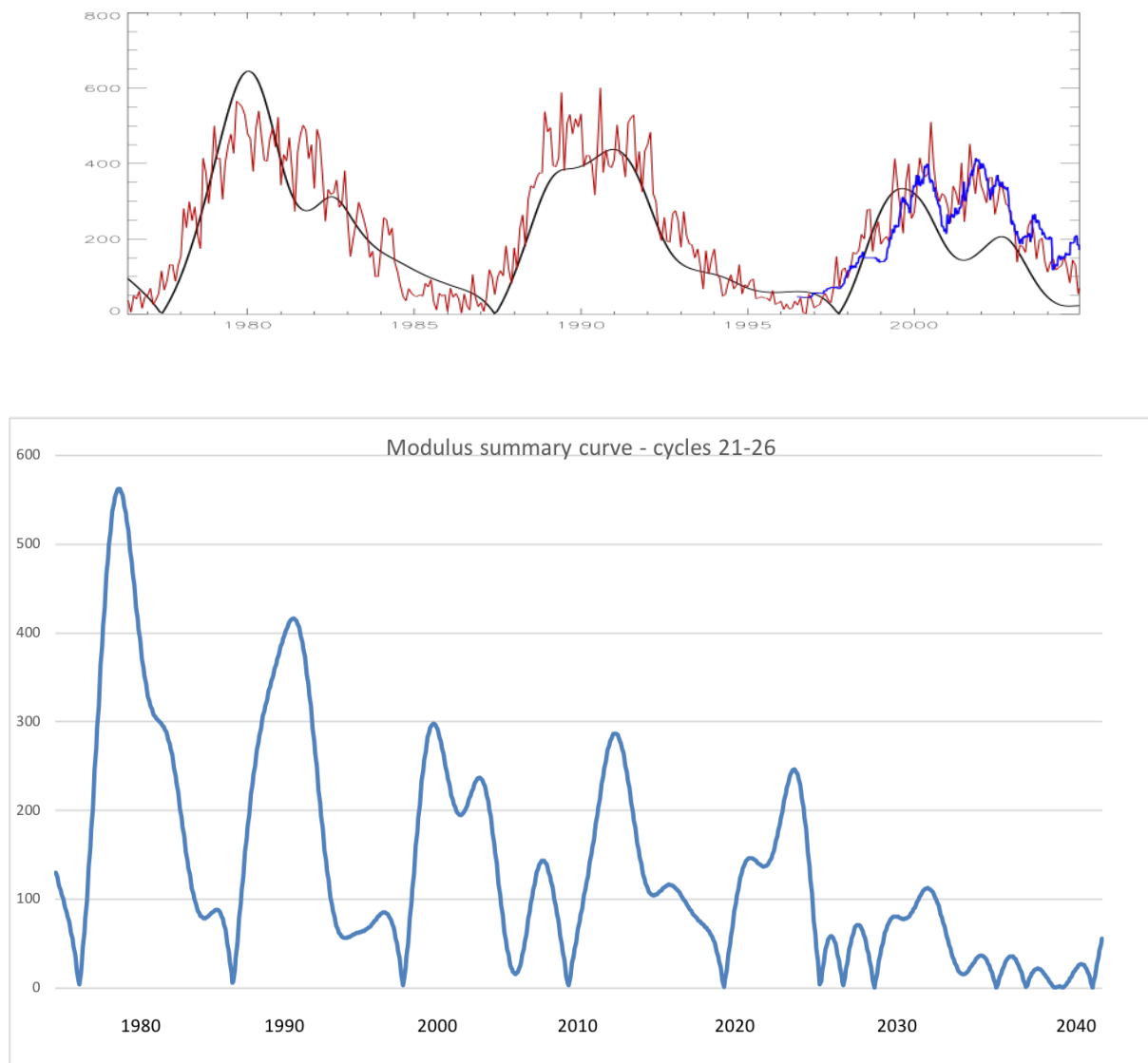
Figure 2. Top plot : The modulus summary curve (black curve) obtained from the summary curve (Figure 1, bottom plot) versus the averaged sunspot numbers (red curve) for the historical data (cycles 21-23). Bottom plot : The modulus summary curve associated with the sunspot numbers derived for cycles 21–23 (and calculated for cycles 24–26 (built from the data obtained by Zharkova et al, 2015)).
