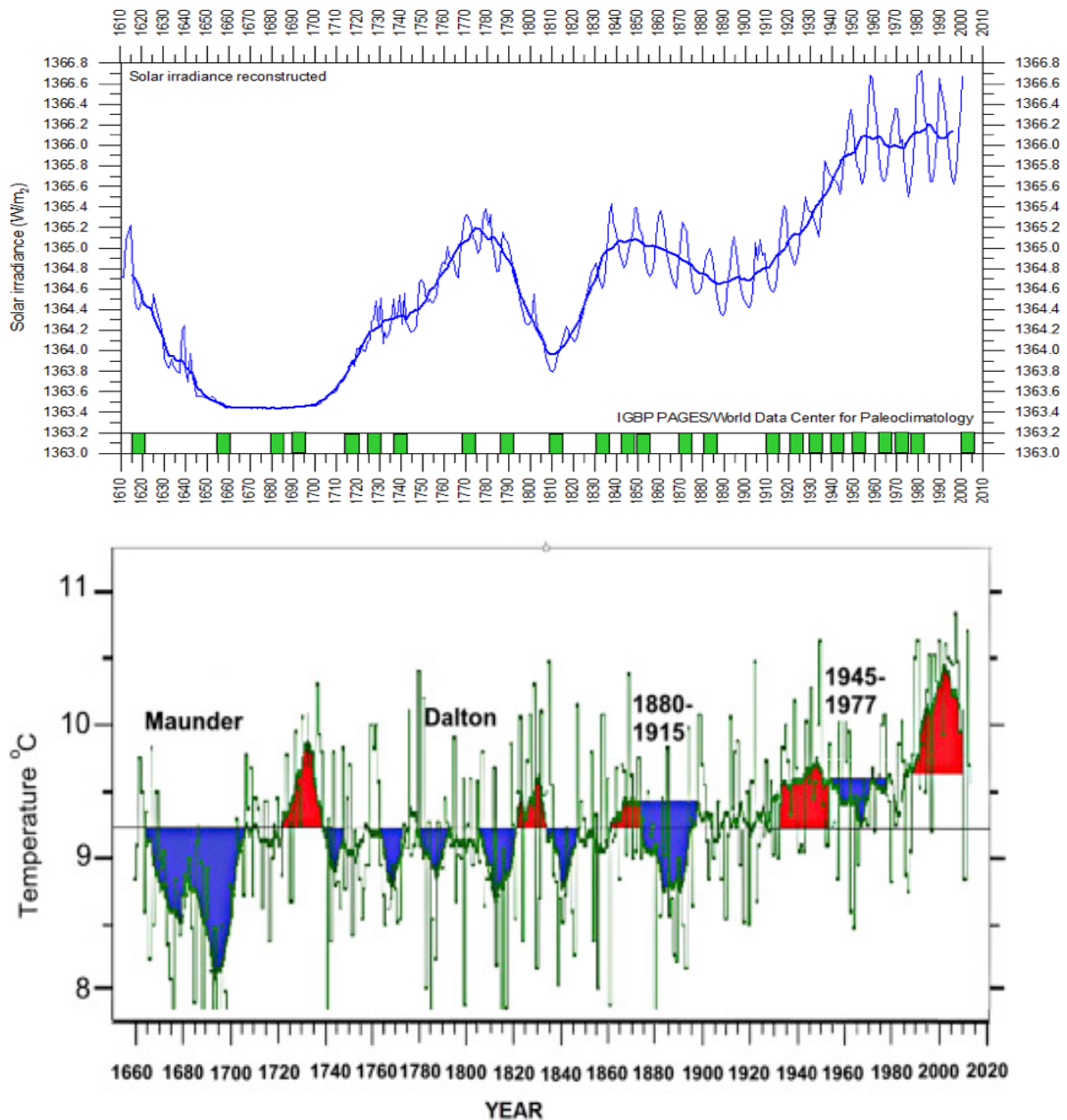
Figure 4. Top plot : restored total solar irradiance from 1600 until 2014 by Lean et al., 1995. Modified by Easterbrook (2016) from Lean, J.L., Beer, J., Bradley, R., 1995. Bottom plot : Central England temperatures (CET) recorded continuously since 1658. Blue areas are reoccurring cool periods; red areas are warm periods. All times of solar minima
