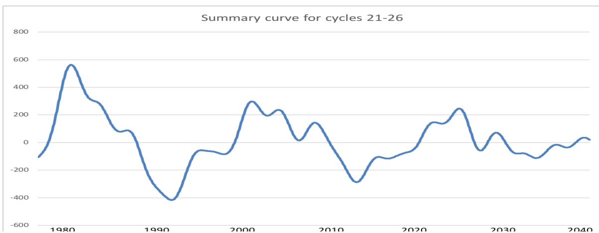
Figure 1. Top plot : two principal components (PCs) of solar background magnetic field (blue and green curves, arbitrary numbers) obtained for cycles 21–23 (historic data) and predicted for cycles 24–26 using the mathematical formulae derived from the historical data (from the data by Zharkova et al., 2015). The bottom plot : The summary curve derived from the two PCs above for the ‘historical’ data (cycles 21–23) and predicted for solar cycles 24 (2008–2019), cycle 25 (2020–2031), cycle 26 (2031–2042) (from the data by Zharkova et al., 2015).
