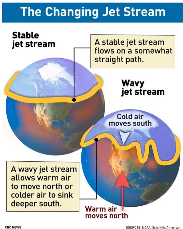
Fig. 10. Cartoon demonstrating formation of wavy jet wiggles in AO/NAO allowing the excursions of the arctic cold air into lower latitudes.
